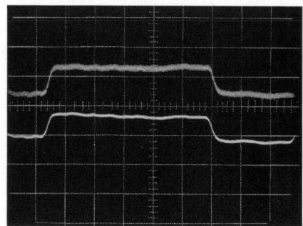
Fig. 8. Double-exposure type oscillogram illustrating a 3 millivolt pulse with no smoothing (upper trace) and using smoothing feature (lower trace) to improve new oscilloscope's already small 2 millivolt rated noise value. External circuit random noise will be similarly improved by smoothing feature.
