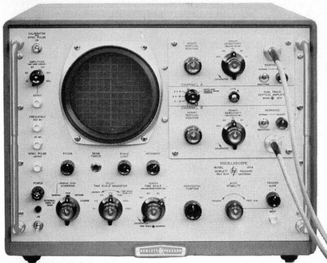
Fig. 6. Panel view of -hp- Model 185A Oscilloscope with Model 187A Dual-Trace plug-in amplifier. Instrument uses new circuit technique, but controls are conventional and include presentation selector for separate or combined - channel displays.
