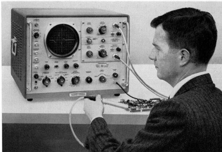
Fig. 1. New -hp- Model 185A/187A Oscilloscope displays signals from 3 millivolts to 2 volts (x10 with adapter) over frequency range up to 500 megacycles. Besides very wide bandwidth and high sensitivity, instrument has several special advantages not found previously in oscilloscopes.
