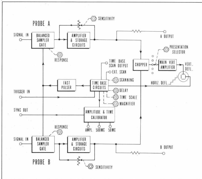
Fig. 7. Basic circuit arrangement of hp-Model 185A/187A Oscilloscope.
